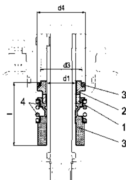
up to 16 bar Cartridge Unbalanced type
