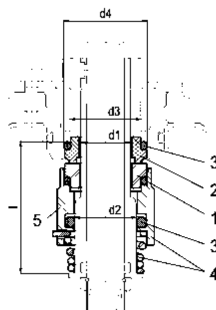
up to 25 bar Cartridge Balanced type
