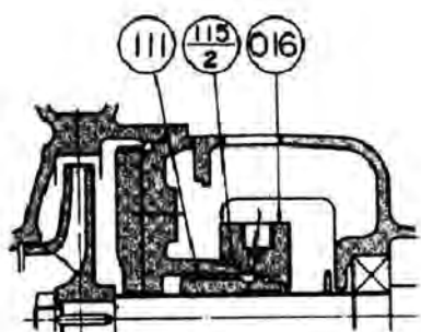
Mechanical seal type (standard)
