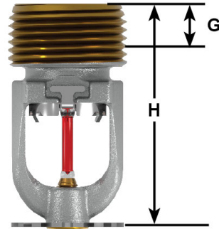
Figure – 2: Dimensions
